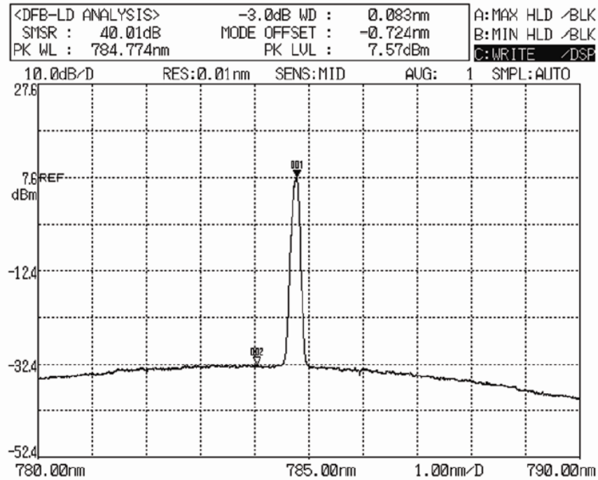
Typical 785 nm SS Laser Spectrum (SMSR > 40 dB)
